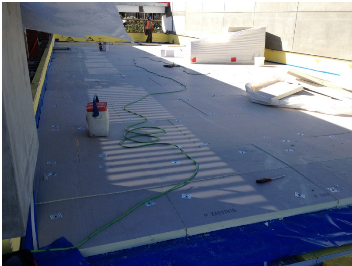
Date: 02/02/16 Progress of roofing installation by JP Witherow in courtyard area. First layer of insulation mechanically fastened to steel deck.
